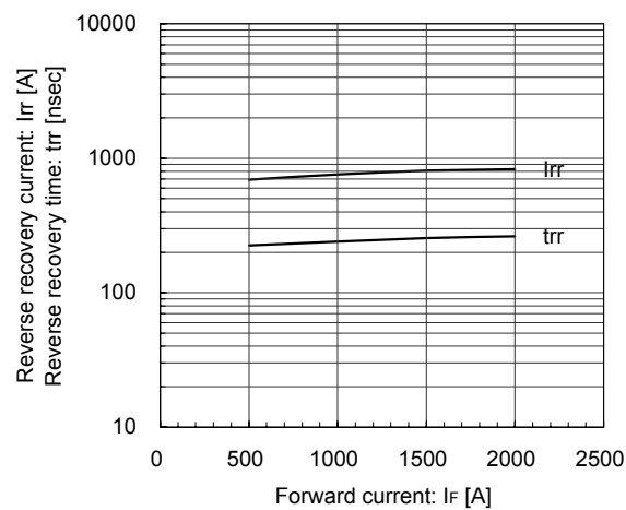
Reverse Recovery Characteristics (typ.) V_{CC}=900V , V_{GE}=\pm 15V , R_G=+1.2/-1.8\Omega , T_J=25^\circ C
