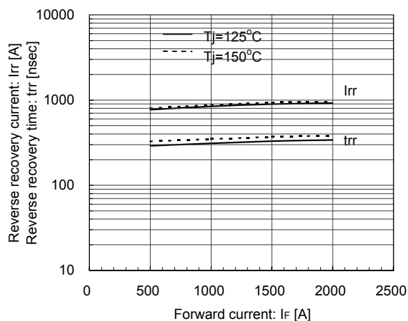
Reverse Recovery Characteristics (typ.) V_{CC}=900V , V_{GE}=\pm 15V , R_G=+1.2/-1.8\Omega , T_J=125^\circ C , 150^\circ C
