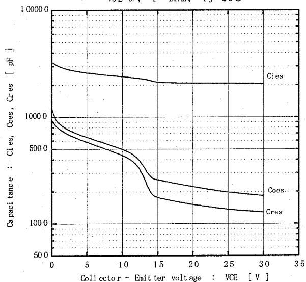
Capacitance vs. Collector-Emiiter voltage (typ.) V_{GE} = 0\text{V} , f = 1\text{MHz} , T_j = 25^\circ\text{C}
