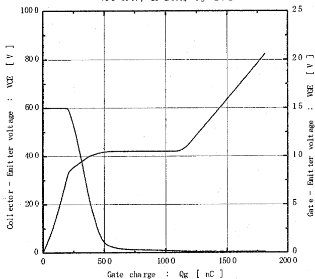
Dynamic Gate charge (typ.) V_{ce} = 600\text{V} , I_c = 200\text{A} , T_j = 25^\circ\text{C}
