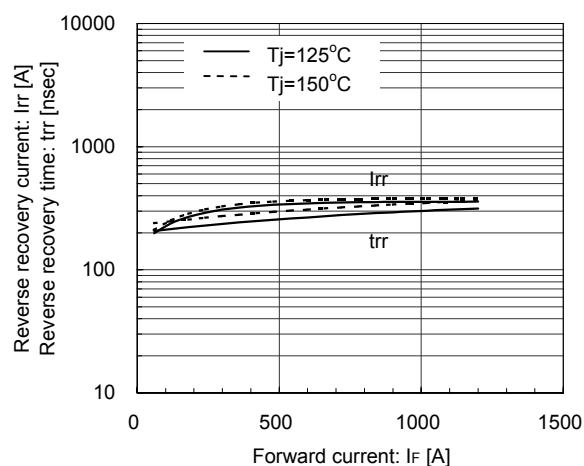
Reverse Recovery Characteristics (typ.) V_{CC}=600\text{V} , V_{GE}=\pm 15\text{V} , R_G=2.4\Omega , T_J=125^\circ\text{C} , 150^\circ\text{C}
