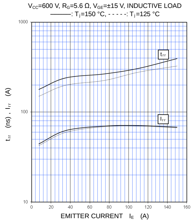
DIODE REVERSE RECOVERY CHARACTERISTICS (TYPICAL)
