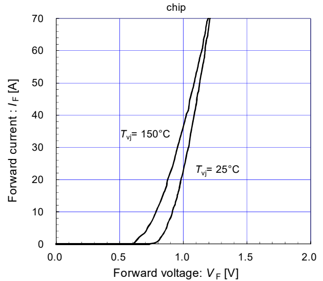
Forward current vs. Forward voltage (typ.) chip
