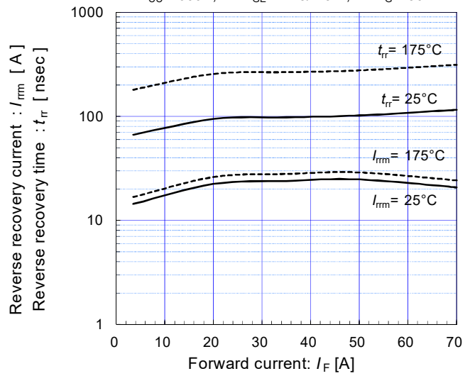
Reverse recovery characteristics (typ.) V_{CC} = 600V , V_{GE} = +15/-15V , R_G = 30\Omega
