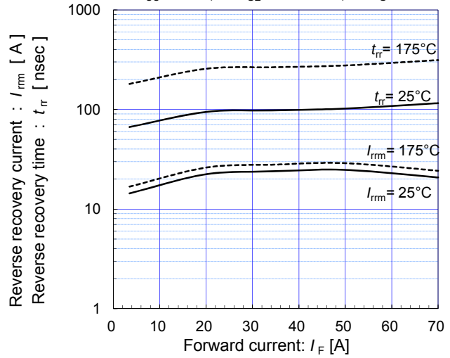
Reverse recovery characteristics (typ.) V_{CC} = 600V , V_{GE} = +15/-15V , R_G = 30\Omega
